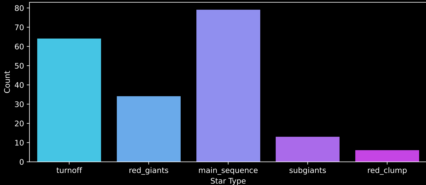
GALAH DR4 Field: [7158] Count plot of Star Type
