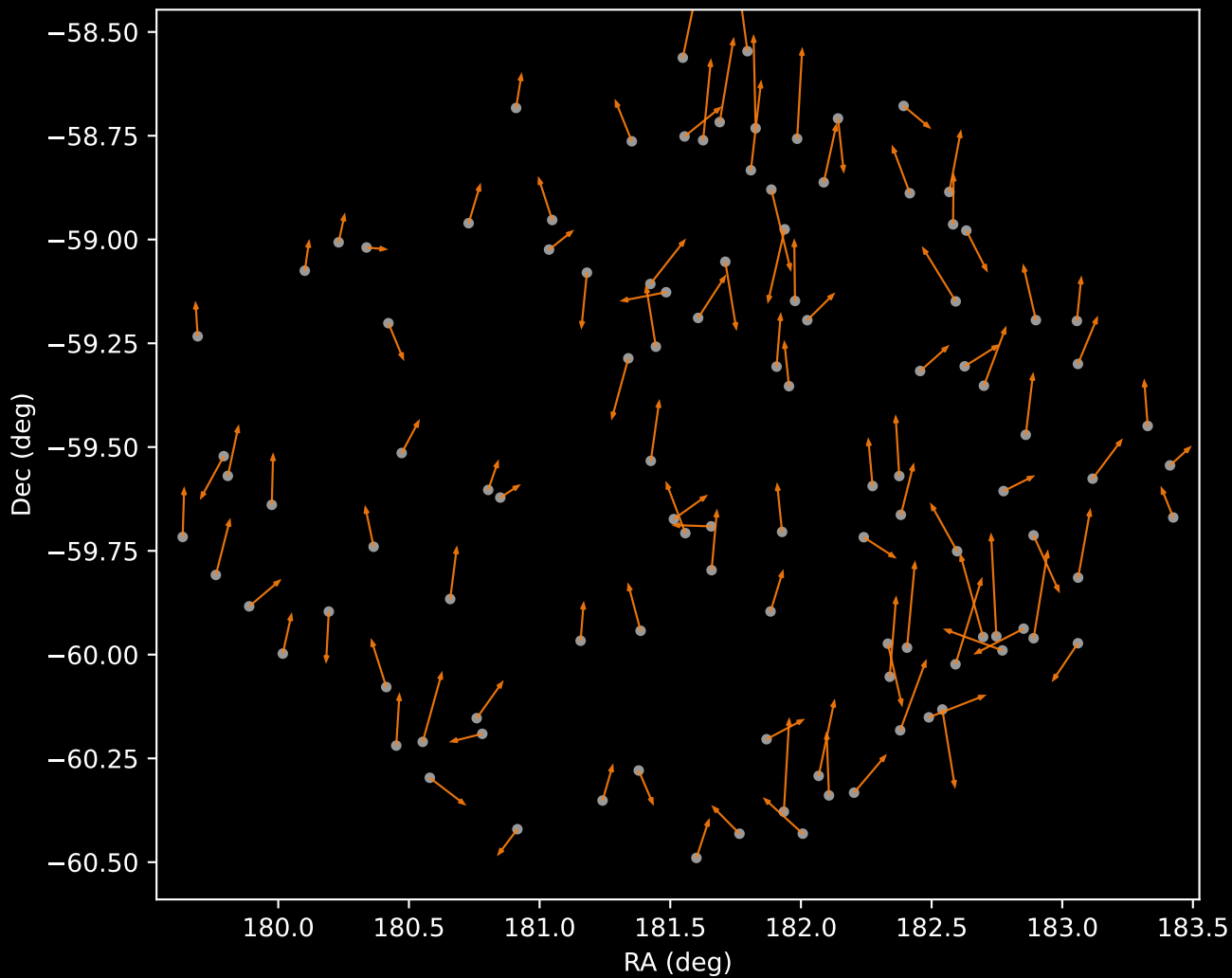
GALAH DR4 Cluster 2 Proper Motion Vectors (n=110)
