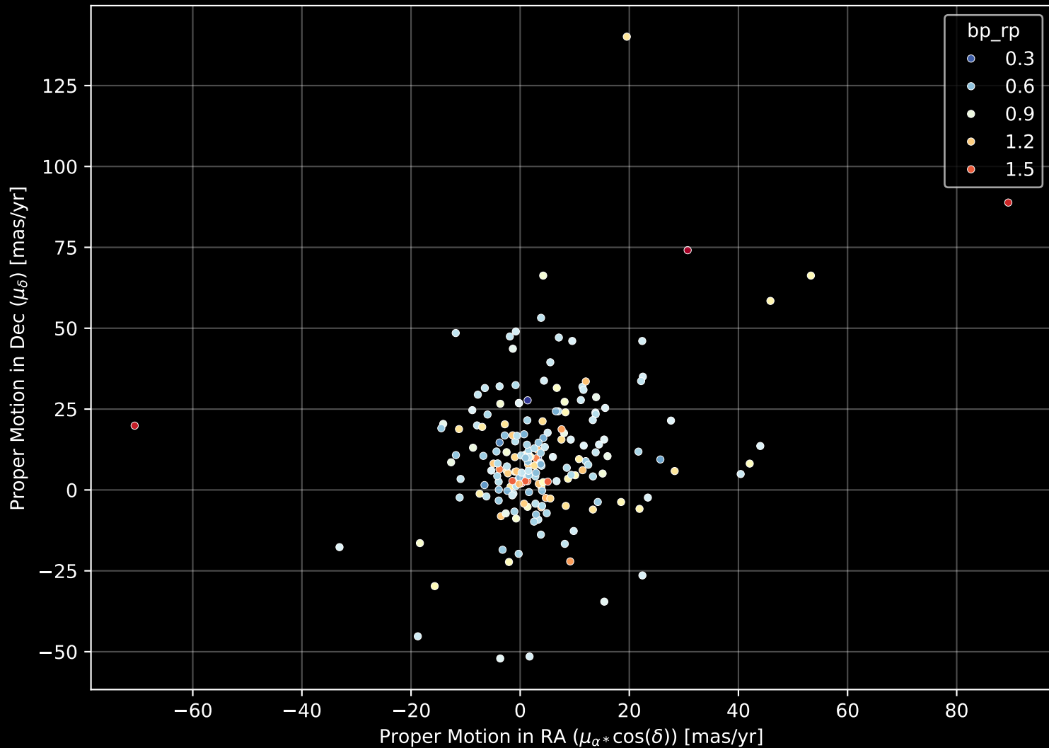
GALAH DR4 Field: [7158] Proper Motion Diagram (n= 196)
